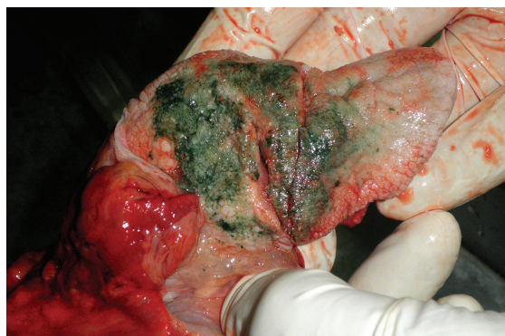
Fig. 3. Greenish coloration of the tongue due to mastication and consumption of mosquito coils. Image taken during autopsy.
