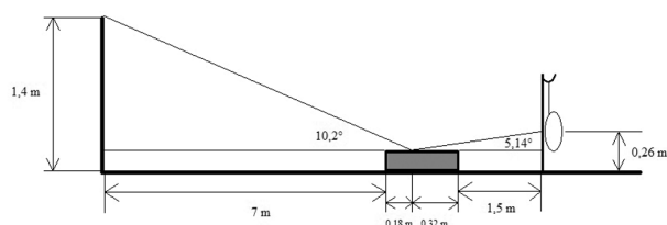
Fig. 3. Scheme of arrangement of the shooting bay (side view) with the particular values marked.
