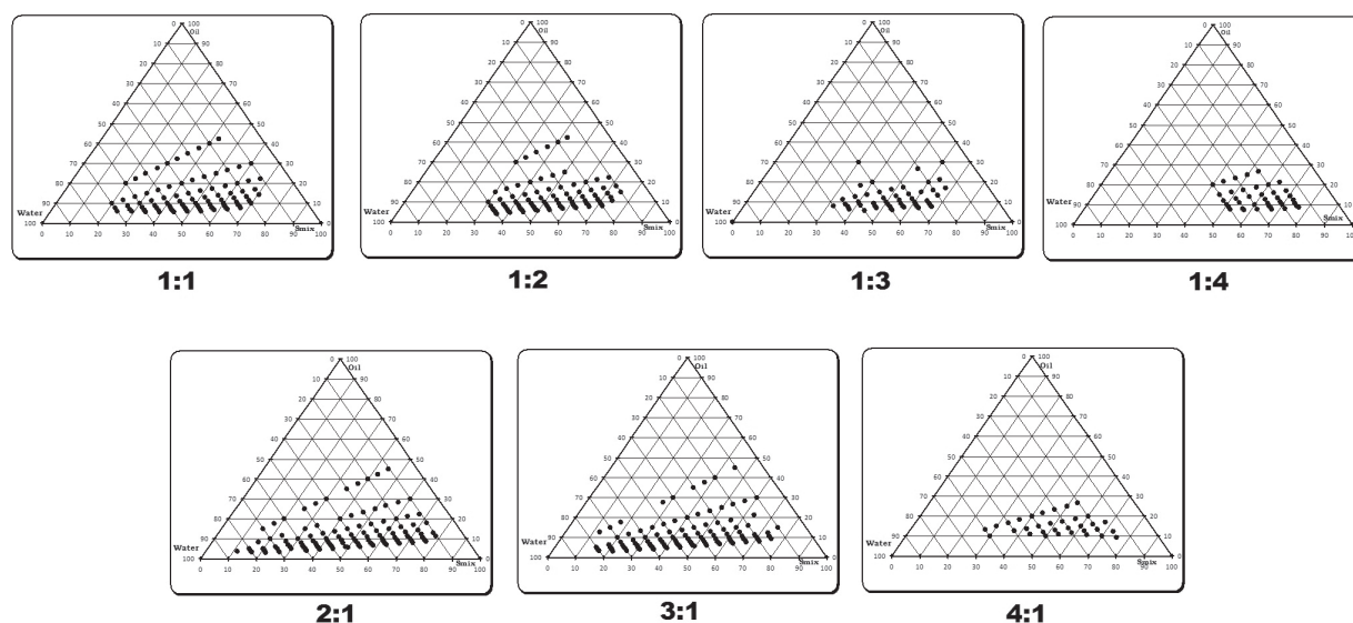
Fig. 3. Pseudoternary phase diagram showing the o/w emulsion region of labrafil, cremophor &amp; plurol oleique at various Smix
